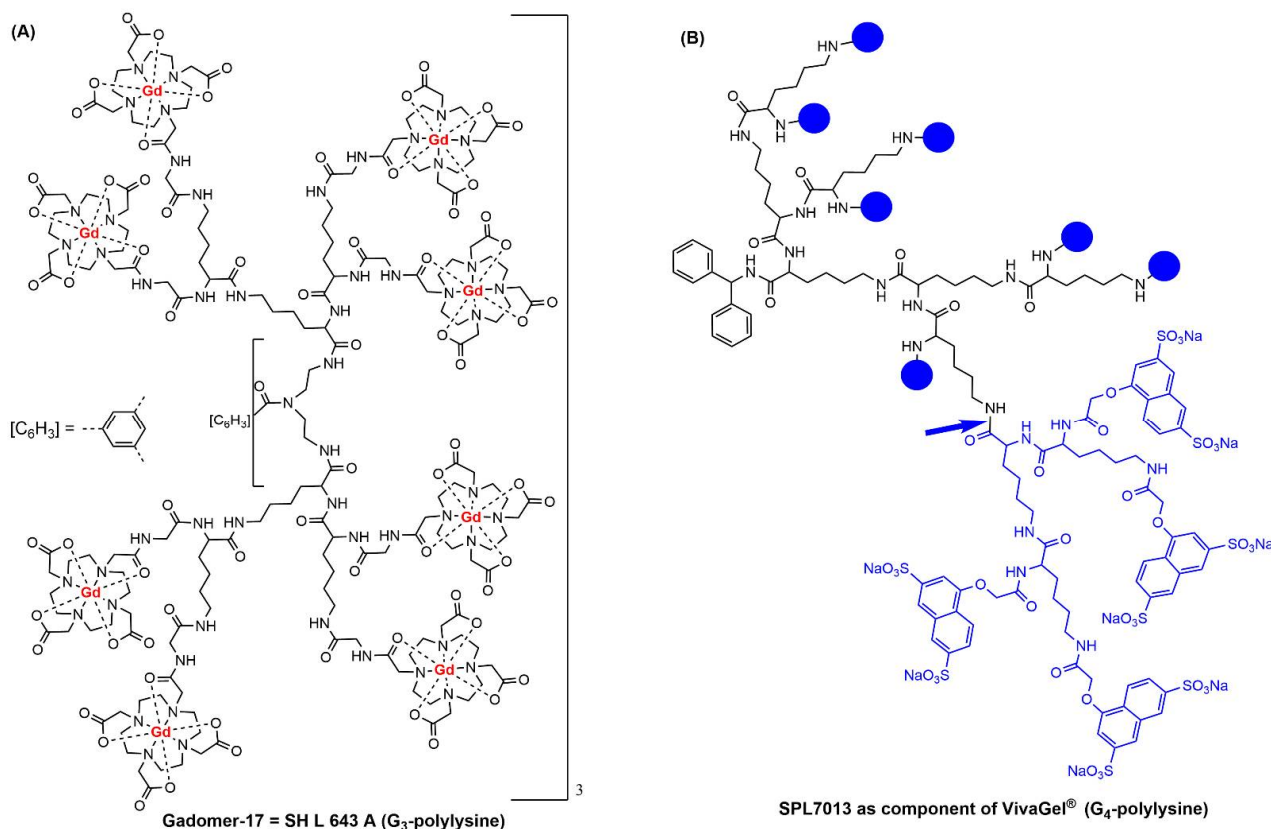
Figure 2. Chemical structure of two poly-L-Lysine dendrimers. (A) Gadomer-17 used as MRI agent. (B) SPL7013, also named Astodrim sodium, the active ingredient in the mucoadhesive gel VivaGel ® ; the blue bowls correspond to the structure that is shown in blue after the blue arrow.
