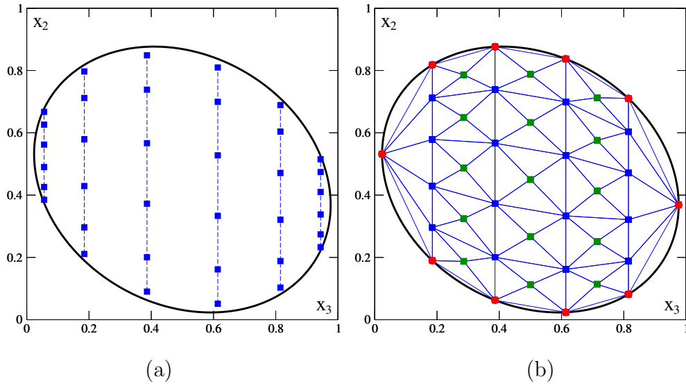
Figure 8: Triangulation of an ellipsoidal cap: (a) nodes position for the volume integration with n_2 = n_3 = 6 (blue squares). The nodes of an internal integration form an array of nodes (dashed lines); (b) first and last elements of internal arrays and first and last arrays are substituted with boundary nodes (red circles). Two couples of consecutive nodes on consecutive arrays are used to define intermediate nodes (green squares) and to form four triangles.
