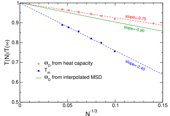
FIG. 6. Variations of the Debye and melting temperatures of iron nanoparticles as a function of inverse particle radius N^{-1/3} , scaled by their bulk limiting value. For the Debye temperature, the two sets of data obtained from the anharmonic heat capacity or the mean square atomic displacement are shown.
