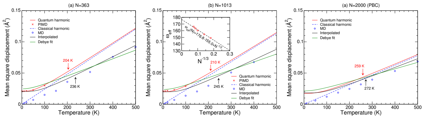
FIG. 3. Mean square atomic displacement obtained for \text{Fe}_N nanoparticles with (a) N = 363 ; (b) N = 1013 ; (c) a 2000-atom bcc sample, from the classical (dashed blue line) and quantum (solid red line) harmonic models, from classical MD (blue circles) and path-integral MD (red crosses, nanoparticles only). The black and green solid lines show the predictions of the interpolation model and the corresponding best Debye fit, respectively, with vertical arrows pointing at the equivalent Debye temperature obtained in the harmonic and anharmonic descriptions. The inset in panel (b) shows the variations of the effective frequency in the interpolation model with increasing inverse particle radius N^{-1/3} .
