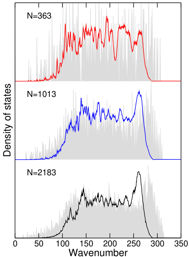
FIG. 1. Vibrational densities of states obtained at 300 K for \text{Fe}_N nanoparticles with 363, 1013, and 2183 atoms. The harmonic densities of states are superimposed in the background as grey lines. No broadening of any kind was imposed to the results.
