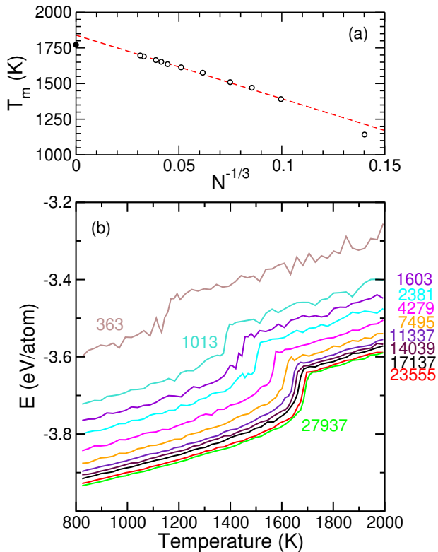
FIG. 5. Melting behavior of \text{Fe}_N nanoparticles from molecular dynamics simulations. (a) Melting temperature as a function of N^{-1/3} , with the bulk value taken from Ref. 26; (b) Internal energy as a function of temperature for particles containing N = 363 – 27937 atoms.
