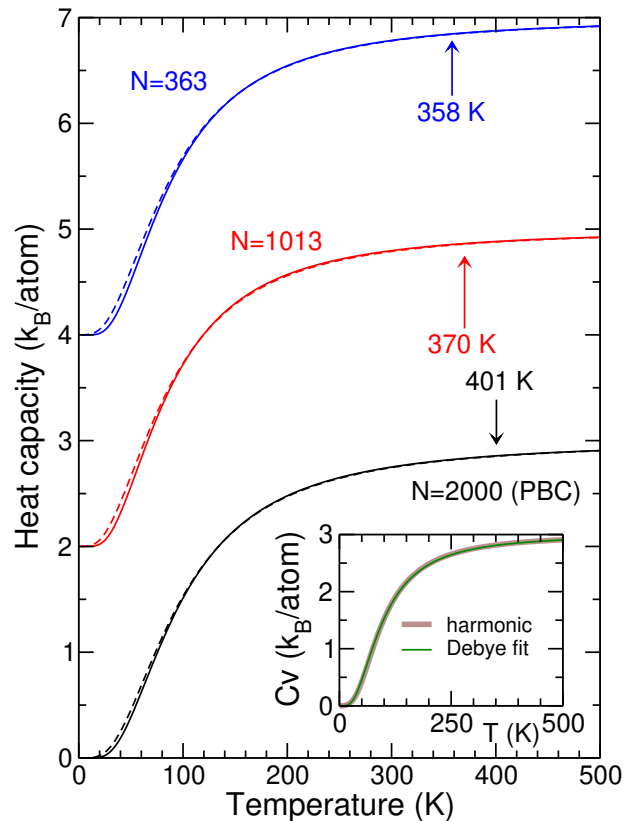
FIG. 2. Lattice canonical heat capacities of \text{Fe}_N nanoparticles with N = 363 and N = 1013 , and for a periodic 2000-atom bcc sample, obtained from the anharmonic vibrational density of states at 300 K (solid lines) and in the harmonic limit (dashed lines). The curves for the two nanoparticles were shifted for clarity, and the vertical arrows mark the value of the Debye temperatures inferred from fitting the anharmonic heat capacities to a Debye model. The inset shows the quality of such a Debye fit against the harmonic prediction for the periodic 2000-atom sample.
