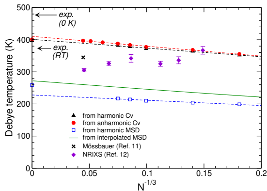
FIG. 4. Debye temperatures of \text{Fe}_N nanoparticles as a function of inverse particle radius N^{-1/3} , obtained from fitting the heat capacity or the mean square atomic displacement using harmonic or anharmonic data, and from available experimental measurements. The experimental Debye temperatures for bulk \alpha iron at 0 K and room temperature are also highlighted by black left arrows, and the simulation results obtained for the periodic 2000-atom bcc sample are also indicated.
