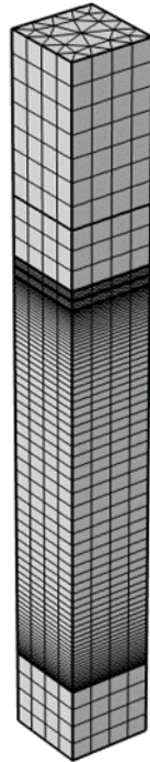
Figure 2: Meshed structure
