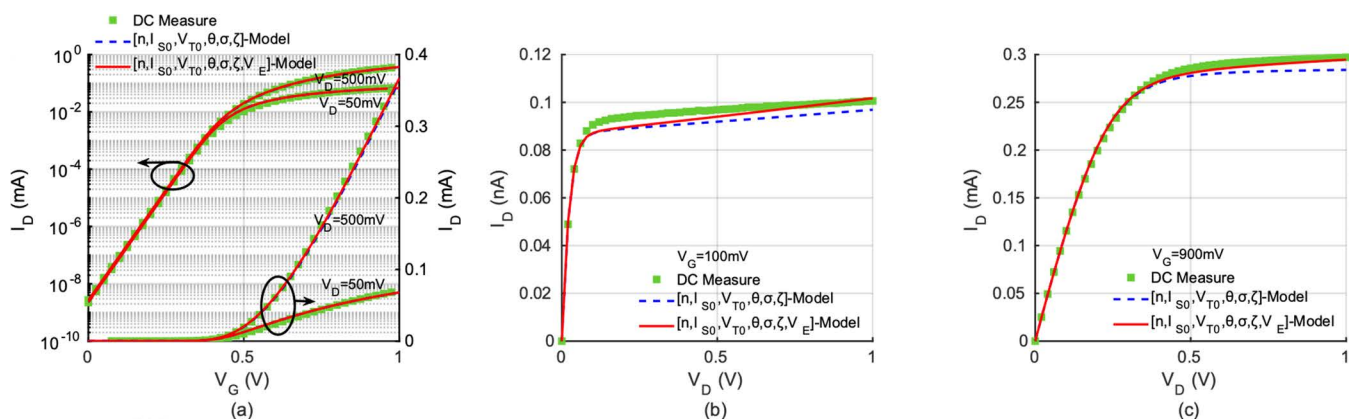
FIGURE 5. L = 150 nm and W = 1 \mu m N-MOS transistor characteristic curves: I_D(V_G) for V_D = 50 mV and 500 mV in linear (right axis) and in semilogarithmic scale (left axis) (a), I_D(V_D) for V_G = 100 mV (b) and for V_G = 900 mV (c): Comparison between measures (green squares) model based on 6 parameters (dashed blue line) and on 7 parameters (red solid line): n = 1.092 , I_{S0} = 1.83 \mu A, V_{T0} = 427 mV, \theta = 0.047 , \sigma = 0.003 , \zeta = 0.06 and V_E = 18.5 V.
