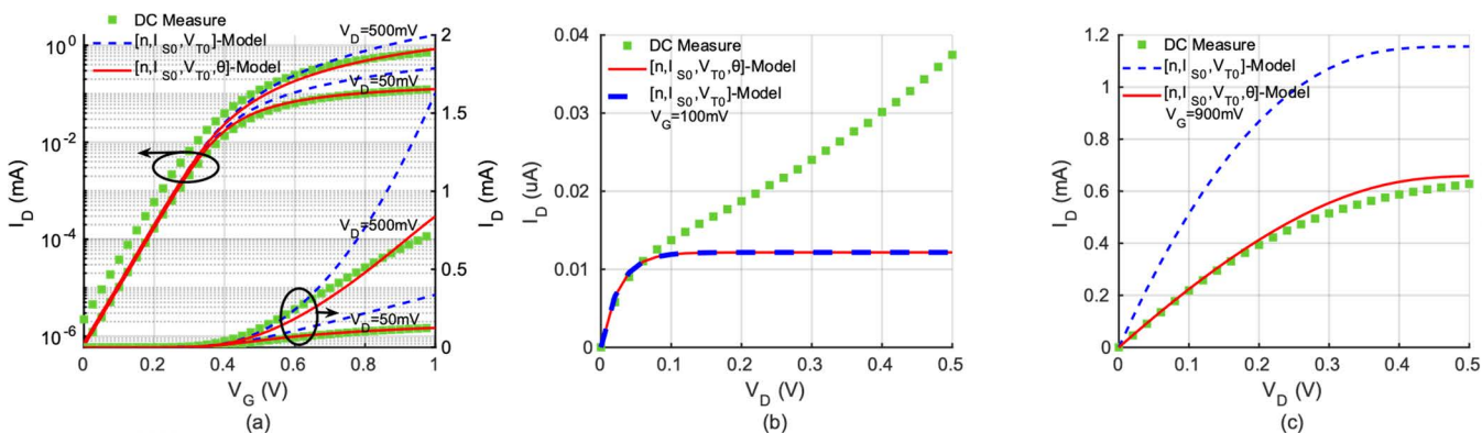
FIGURE 2. L = 30 nm and W = 1 \mu m N-MOS transistor characteristic curves: I_D(V_G) for V_D = 50 mV and 500 mV in linear (right axis) and in semilogarithmic scale (left axis) (a), I_D(V_D) for V_G = 100 mV (b) and for V_G = 900 mV (c): Comparison between measures (green squares) model based on 3 parameters (dashed blue line) and on 4 parameters (red solid line): n = 1.377 , I_{S0} = 5.9 \mu A, V_T = 380.3 mV and \theta = 0.115 . Note that for (b) there is no change between both models based on 3 and 4 parameters, as the effect of mobility reduction ( \theta ) appears only in strong inversion.
