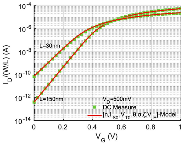
FIGURE 10. I_D/(W/L) (V_G) curve: Comparison of a long ( L = 150 nm) and a short ( L = 30 nm) channel NMOS transistor, DC measures (green squares) and 7-parameters model (red solid line). The short channel effects: slope factor, threshold voltage, velocity saturation and series resistance are clearly visible in this curve.
