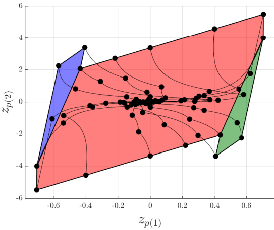
Fig. 4. Trajectories starting at the boundary of \Omega_{i,x_p} .
