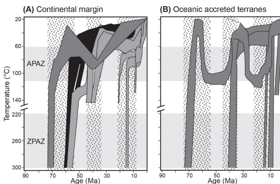
Fig. 8. Thermal history of the Ecuadorian Andes (after Spikings et al., 2010). Dotted areas: inferred exhumation periods. (A): Continental margin. Light grey: northern Eastern Cordillera; black: southern Eastern Cordillera; dark grey: Amotape Massif. (B) Oceanic accreted terranes (Western Cordillera). APAZ and ZPAZ: Apatite and Zircon partial annealing zone, respectively.
