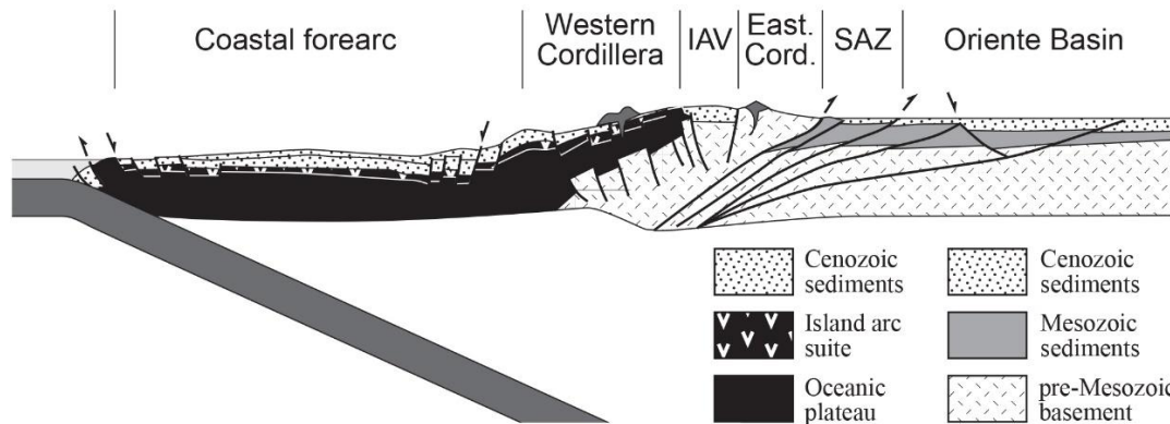
Fig. 6. Schematic cross section of the Ecuadorian Andes assuming the obduction of a single accreted terrane (simplified from Vallejo et al., 2019). Compare with Fig. 11 and 13. IAV: Inter-Andean Valley; SAZ: Sub-Andean Zone.
