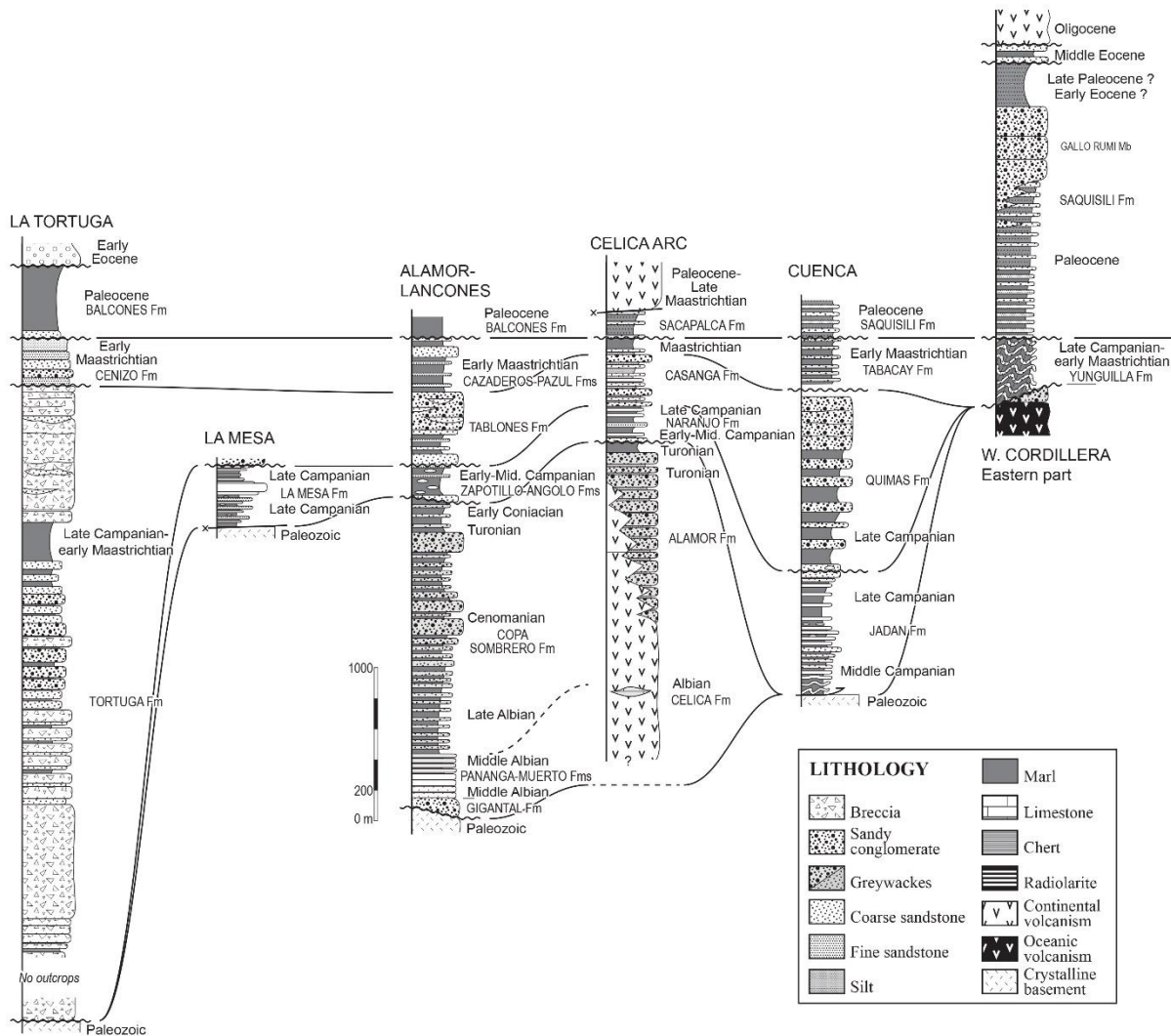
Fig. 3. Simplified stratigraphic succession of late Cretaceous-Paleogene age from the forearc zones of northwestern Peru (left) to central Ecuador (right) (from Jaillard et al., 1996; 1999; 2004; 2005).
