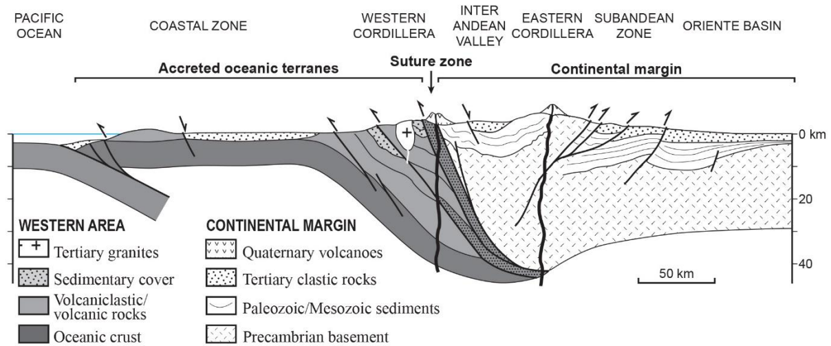
Fig. 11. Schematic cross section of the Ecuadorian Andes (adapted from Mégard, 1989). Note the western, west-verging wedge made of oceanic terranes, and the eastern, east-verging wedge, made of continental rocks. Compare with Fig. 6.
