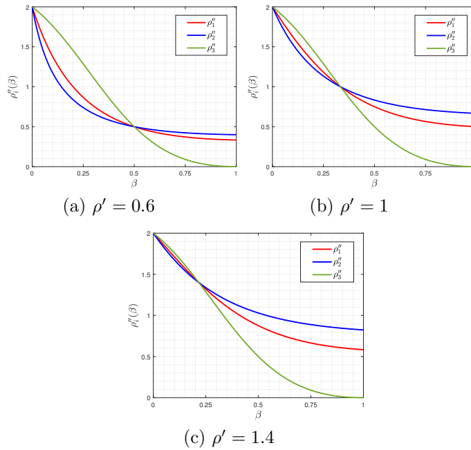
Figure 1: Upper bound of the relaxation parameters \rho''_i(\beta) ( i = 1, 2, 3 ) given in (4.5), (4.15) and (4.18) as functions of inertial step upper bound \beta > 0 .
