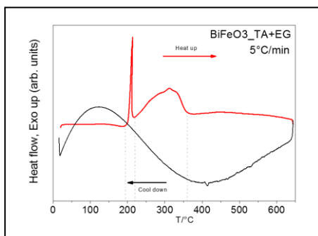
Figure 1. Heating and cooling ramps of DSC experiments using \text{BiFeO}_3 precursor powders, synthesized using tartaric acid (TA) and ethylene glycol (EG). The decomposition heat exchange of tartaric acid, ethylene glycol and the esterification network correspond to the exothermic contributions observed in the heating ramp around 200°C and 350°C.
