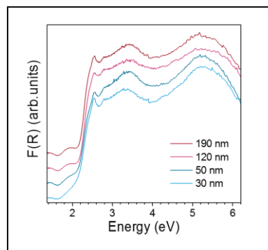
Figure 2. Room temperature UV-Vis absorption spectra of different size \text{BiFeO}_3 samples derived from the diffuse reflectance (R) spectra using Kubelka-Munk functions F(R) on pure phase nanopowders nanoparticle size indicated in the legend.
