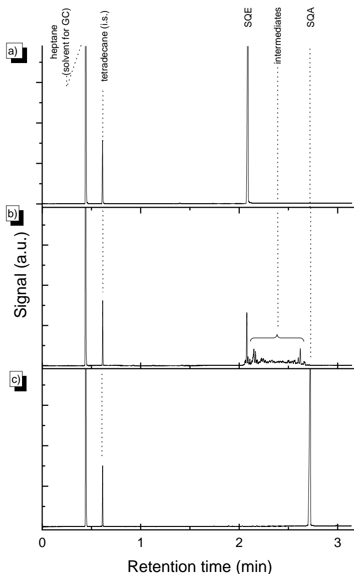
Figure 2. Comparison of the GC/FID chromatograms as the function of reaction progress. a) initial composition of reaction mixture; b) reaction mixture at 85% conversion, 1 h; c) final composition of the reaction mixture after 9 h (Conversion >98%). Reaction conditions: H 2 20 bar; 120 °C; liquid phase 80 mL of solvent-free SQE (2.03 M) with tetradecane as internal standard (0.1 M); Pd 0.08 mol % (280 mg of 5 wt % Pd/ \gamma -Al 2 O 3 ), 120 °C. Heptane was used to dilute the reaction mixture for GC analysis. (See supporting information in Figures S1 to S4 for full-scale chromatograms).
