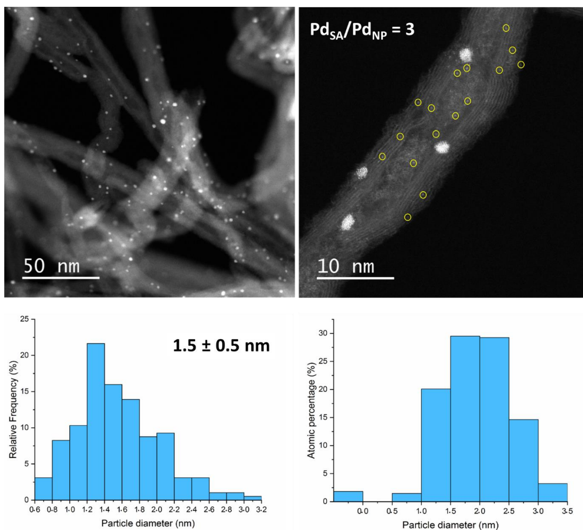
Figure 4. STEM-HAADF micrographs and particle size distribution are based on total particles and total atoms for Pd/CNT catalyst.
