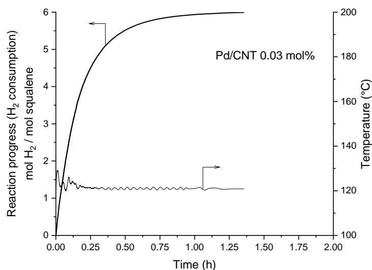
Figure 5. H 2 consumption and temperature as the function of time. Reaction conditions: H 2 20 bar; 120 °C; liquid phase 80 mL of solvent-free SQE (2.03 M) with tetradecane as internal standard (0.1 M); Pd 0.03 mol % - 300 ppm (270 mg of 2.04 w% Pd/CNT).
