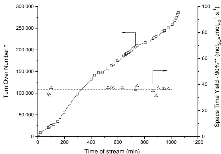
Figure 8. Turn Over Number (TON) and Space Time Yield at 90% SQA yield (STY-90%) as the function of time on stream. *TON was defined as six times the amount of SQA produced. Intermediates were not considered (see text). **STY-90% was determined for reference recurrent experimental conditions (see text). Reaction conditions: effective reactor volume (V r ) 5.8 mL; 95.7 mg of 2.04wt% of Pd/CNT coated on Fecralloy OCF (Foamet 400µm); H 2 30 bar; SQA concentration between 0.33 and 2.03 M (solvent-free) with tetradecane as internal standard (0.1 M); temperature between 120 and 180 °C; Q G between 0.16 and 1.2 NL.min -1 ; Q L between 0.4 and 8 mL.min -1 . Lines are guides to the eyes. See supporting information Figure S 11 for details.
