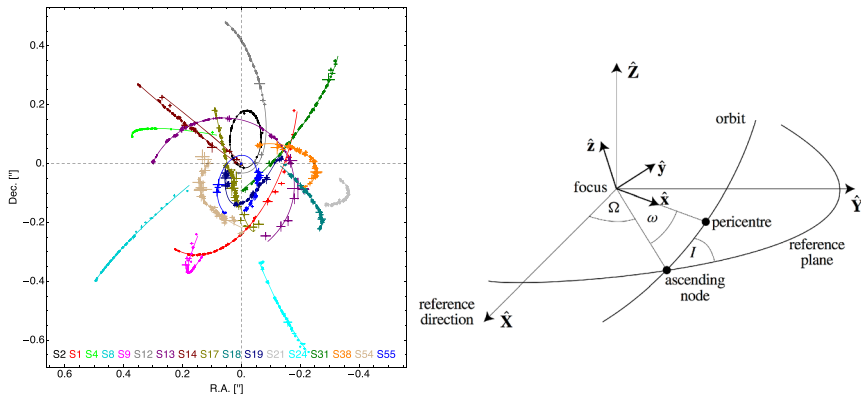
Fig. 31 Keplerian orbits around an MBH. Left: Detailed observations of the Keplerian dynamics of the S-stars in the vicinity of Sgr A* ( \sim 10 mpc) from Gillessen et al. (2017). At leading order, orbits take the form of closed ellipses, because the central MBH dominates the gravitational potential. Right: Illustration of the Keplerian orbital elements from Murray and Dermott (1999)
