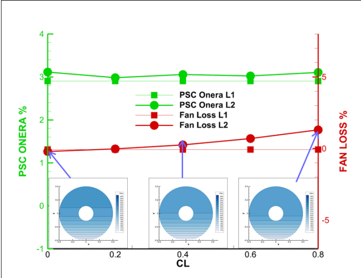
Figure 21: Common Inlet concept - PSC and fan losses.
