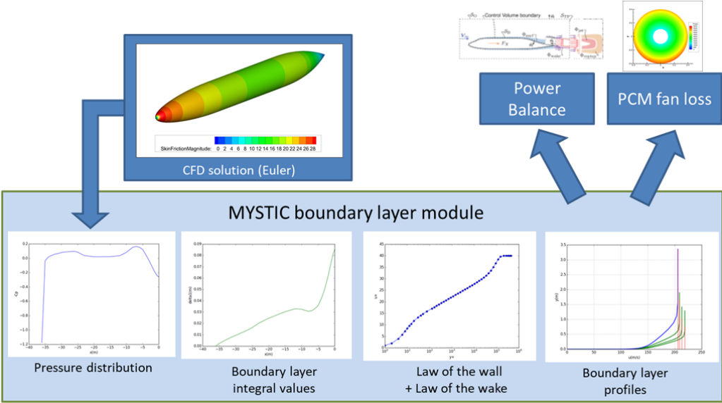
Figure 10: Level 2 BLI module - Schematic view.
