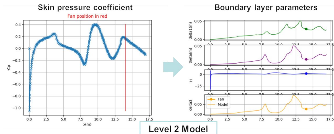
Figure 20: Common Inlet concept - Integral Boundary Layer method.
