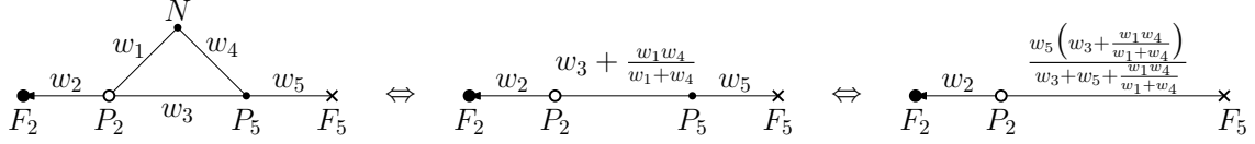
Figure 6: Notation for the proof of (6.1), and calculation of p_{22}(w) , the probability of reaching F_2 before F_5 starting from P_2 .
