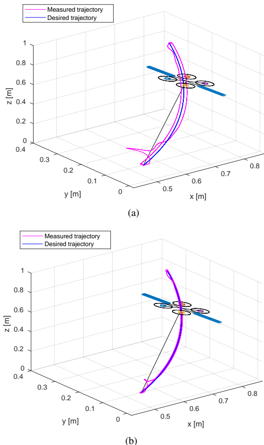
Fig. 5: System's 3D trajectory at V_w = 5\text{m/s} (a) without actuators compensation, (b) with actuators compensation
