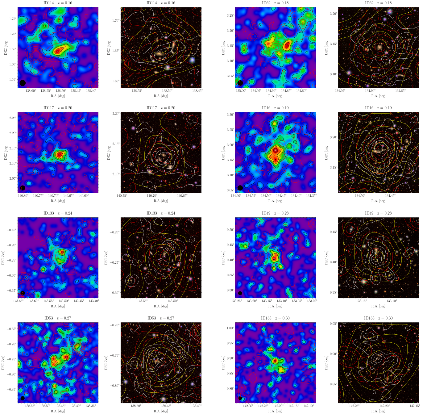
Fig. B.1: Left : Galaxy density maps (16 × 16 arcmin) centred on the HSC shear-selected cluster positions with a unique eFEDS match. Overlaid in red are X-ray contours, which were obtained by smoothing the raw X-ray image in the 0.5 – 2.0 keV energy band with a Gaussian of 24 arcsec. The black circles in the lower-left corners show the smoothing scale, FWHM = 200 kpc. Right : HSC-SSP optical images centred on the HSC shear-selected cluster positions. The 8 \times 8 arcmin optical images of the central region are created using the z , i , and r bands. X-ray contours are shown in red, galaxy density contours in white (they are the same contours as the black ones in the corresponding galaxy density maps), and weak-lensing mass contours in yellow.
