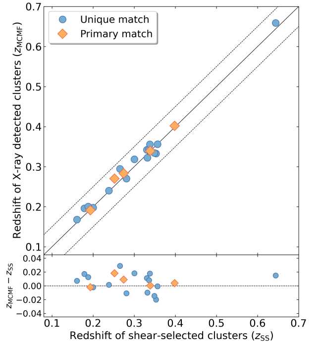
Fig. 3. Top: comparison between the assigned redshift of the shear-selected and the X-ray detected clusters. In blue, clusters are shown that have one unique match between the catalogues within 5 arcmin and with a redshift difference |\Delta z| < 0.1 . The orange points display primary matches for clusters with multiple matches. Primary matches correspond to the most X-ray luminous (and in most cases the closest) eFEDS counterpart. The solid black line shows the 1:1 relationship, and the dotted black lines, a \pm 0.05 offset from this relation. Bottom: difference between redshifts.
