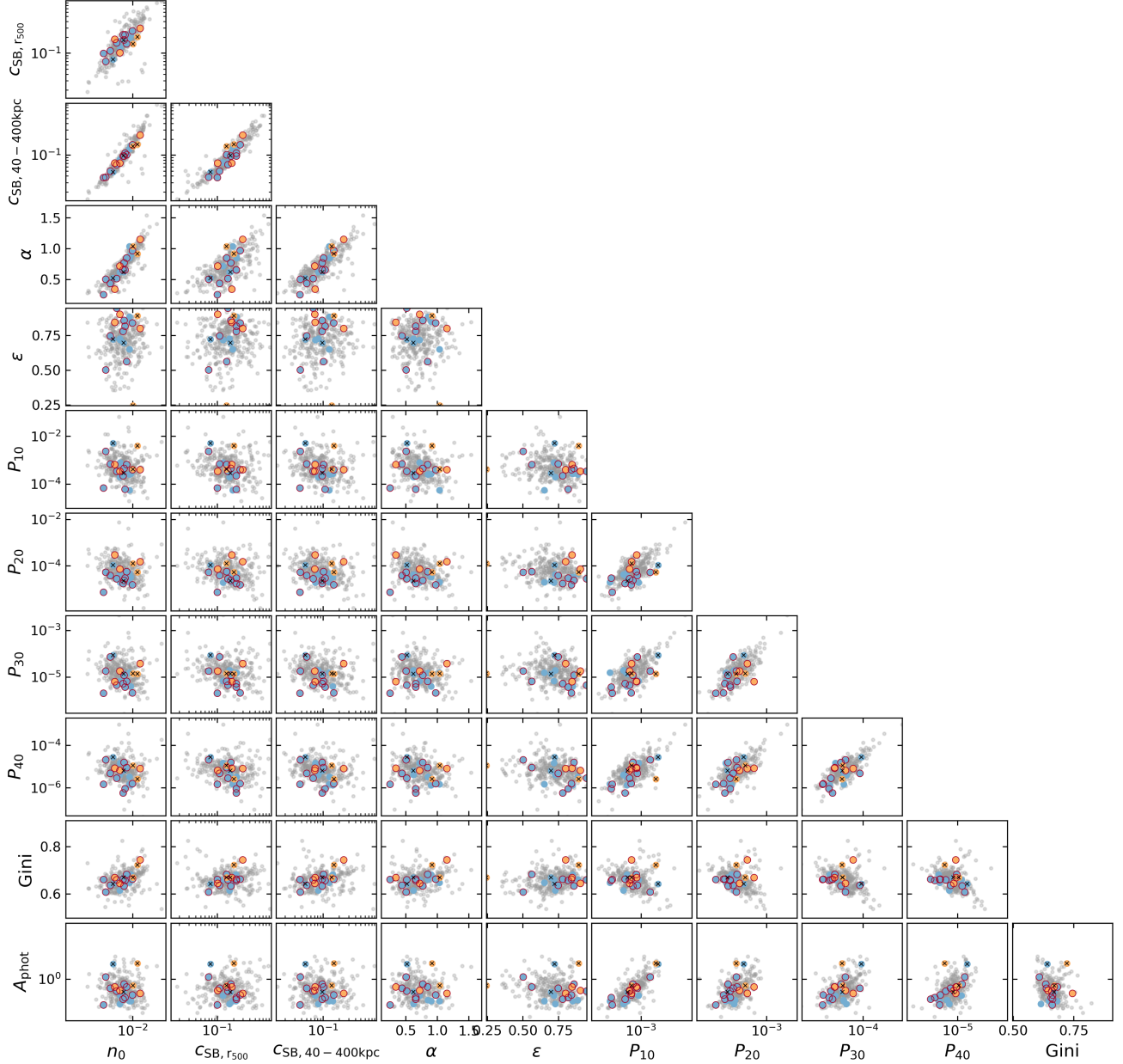
Fig. C.1: L_X and z corrected X-ray morphological parameters obtained within r_{500} in the parameter-parameter planes. Grey points represent the eFEDS sample discussed in Ghirardini et al. (2022) . Blue-filled circles show the shear-selected clusters with a unique eFEDS match; filled-orange circles display weak-lensing peaks with a primary eFEDS counterpart. Points with a red ring around have multiple-peaks, which were classified as such using the peak-finding method described in section 4.3.2. Shear-selected clusters that fall out from the Ghirardini et al. (2022) selection are marked with a black cross. Errors are omitted for clarity purposes. Please refer to Ghirardini et al. (2022) for the error visualisation.
