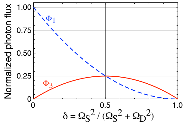
Figure 3. Expected stationary photon fluxes \Phi_1(z \rightarrow \infty) (blue dashed line, signal frequency) and \Phi_3(z \rightarrow \infty) (red solid line, target frequency) as a function of the overall photon losses \delta . The curves are normalized with respect to the initial photon flux at the signal frequency ( \Phi_1(z=0) = 1 ).
