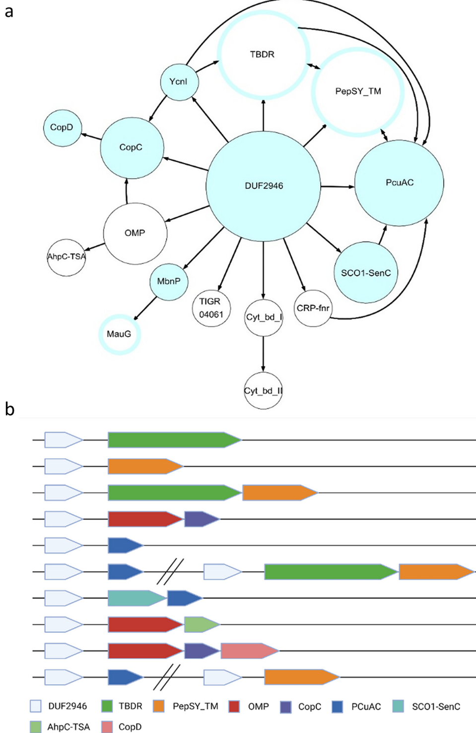
FIG 7 Genetic environments of cruR homologs. a, DUF2946-coding genes were systematically found in first positions of putative operons that comprise genes coding for proteins of the indicated families, represented by circles whose sizes correspond to the current numbers of occurrences of each protein type in those operons (large circle, 400 to 1000; medium-size, 50 to 399; small circles, 1 to 49). Blue-filled circles represent protein families involved in copper homeostasis or utilization, and those surrounded by blue lines represent families some members of which are found in copper-related operons, while others may be involved in distinct processes. The arrows indicate the order of the genes in the putative operons. b, Representation of the most frequent genetic organizations. Parallel bars separate potentially distinct transcriptional units at the same locus.
