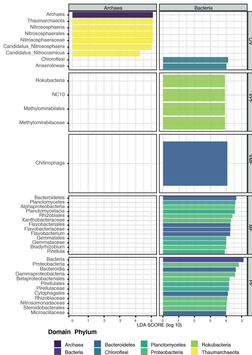
FIGURE 8. Results of LEfSe for archaeal/bacterial taxonomic composition.
