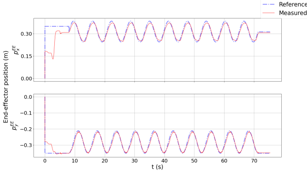
(a) End-effector position in the x, y -plane of the \heartsuit frame for the horizontal surface sanding
