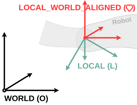
Fig. 1: Representation of the 3 reference frames
