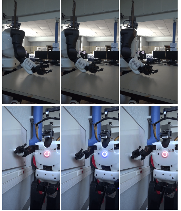
Fig. 3: Screenshot of the horizontal (top) and vertical (bottom) sanding tasks.
