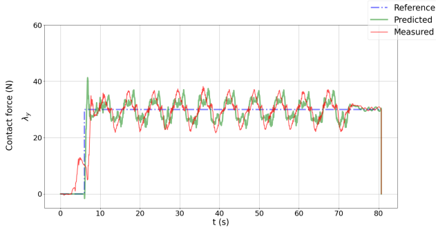
(b) Contact force in the y direction ( \heartsuit frame) for the sanding task on a vertical board
