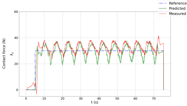
(a) Contact force in the z direction ( \heartsuit frame) for the sanding task on a horizontal table
