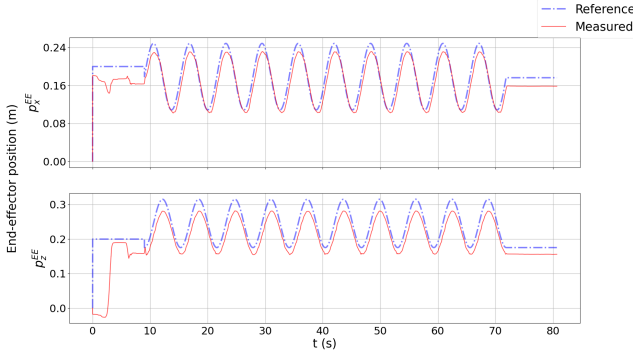
(b) End-effector position in the x, y -plane of the \heartsuit frame for the vertical surface sanding
