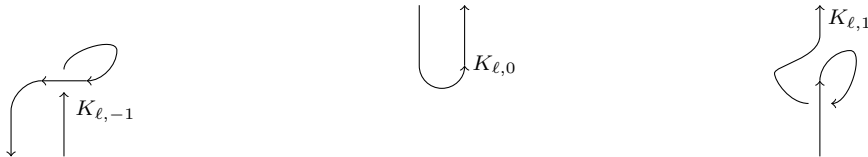
Figure 12: Long tangle representatives
