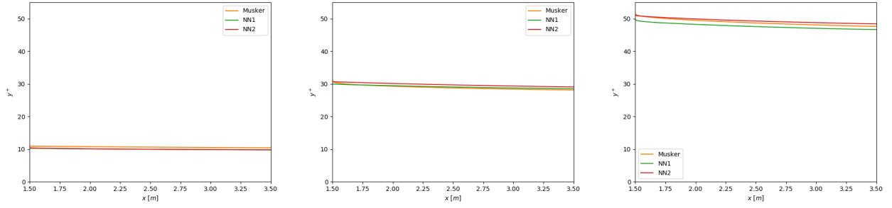
(a) Wall distance at first RANS computed cell (mesh labeled as y^+ \approx 10 ). (b) Wall distance at first RANS computed cell (mesh labeled as y^+ \approx 30 ). (c) Wall distance at first RANS computed cell (mesh labeled as y^+ \approx 50 ).
