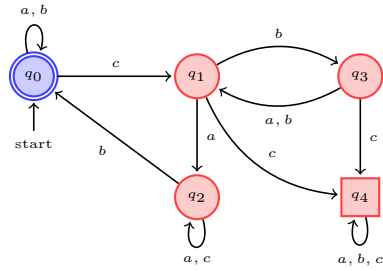
Fig. 2: Property \varphi of Example 1
