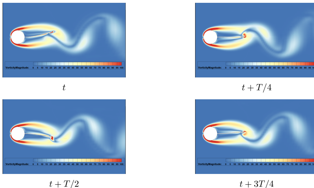
Figure 7: Fluid-structure interaction between the vortices in the wake of the cylinder and the flexible beam during one period. Visualization of the vorticity magnitude.
