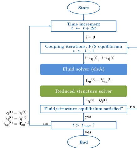
Figure 6: Flowchart of the partitioned coupling between the fluid solver elsA and the nonlinear reduced structural solver. We use the notation \mathbf{f}_{ag} = \mathbf{V}^T \mathbf{f}_a .
