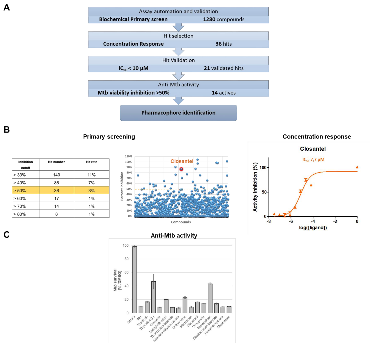
Fig. 2: Screening the FAAL32 activity identifies hits active on Mtb growth. A. Workflow of the chemical library screening against FAAL32 activity and on Mtb viability in vitro . B. Primary screening of the chemical library at 33 \mu M and concentration response curve for the hit closantel. C. Hit activity on Mtb viability in monodose at 10 \mu M . The negative (DMSO) and positive (Isoniazid INH) controls of inhibition are indicated. Mtb survival is calculated relative to DMSO control. Tiratricol: Tiratricol,3,3',5-triiodothyroacetic acid.
