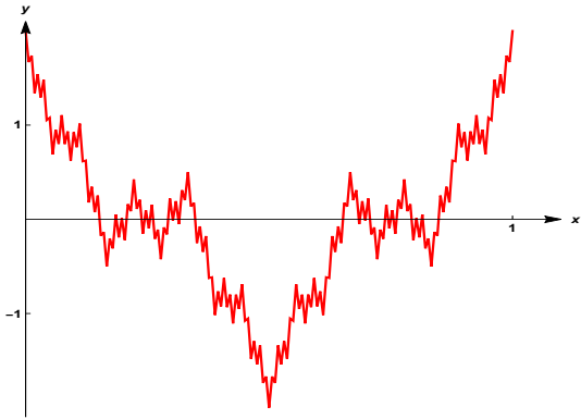
(e) The prefractional graph \Gamma_{\mathcal{W}_4} , in the case when \lambda = \frac{1}{2} and N_b = 3 .
