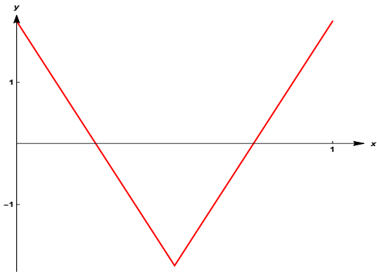
(a) The prefractional graph \Gamma_{\mathcal{W}_0} , in the case when \lambda = \frac{1}{2} and N_b = 3 .
