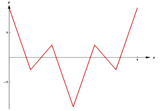
(b) The prefractional graph \Gamma_{\mathcal{W}_1} , in the case when \lambda = \frac{1}{2} and N_b = 3 .
