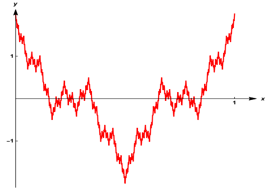
(f) The prefractional graph \Gamma_{\mathcal{W}_5} , in the case when \lambda = \frac{1}{2} and N_b = 3 .
