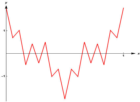
(c) The prefractional graph \Gamma_{\mathcal{W}_2} , in the case when \lambda = \frac{1}{2} and N_b = 3 .
