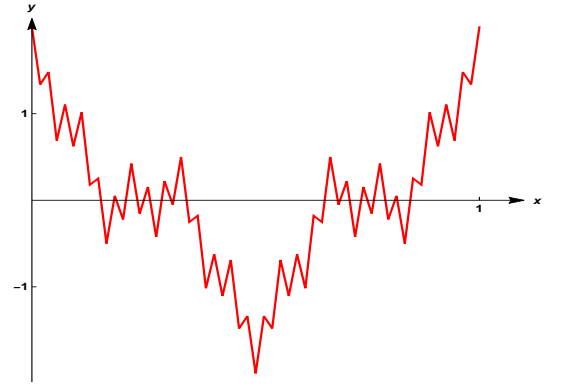
(d) The prefractional graph \Gamma_{\mathcal{W}_3} , in the case when \lambda = \frac{1}{2} and N_b = 3 .
