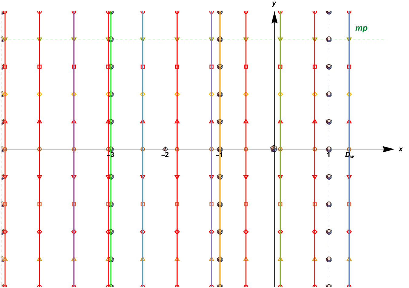
Figure 5: The Complex Dimensions of the Weierstrass Curve. The nonzero Complex Dimensions are periodically distributed (with the same period \mathbf{p} = \frac{2\pi}{\ln N_b} , the oscillatory period of \Gamma_{\mathcal{W}} ) along countably many vertical lines, with abscissae D_{\mathcal{W}} - k(2 - D_{\mathcal{W}}) and 1 - 2k , where k \in \mathbb{N} is arbitrary. In addition, 0 and -2 are Complex Dimensions of \Gamma_{\mathcal{W}} .
