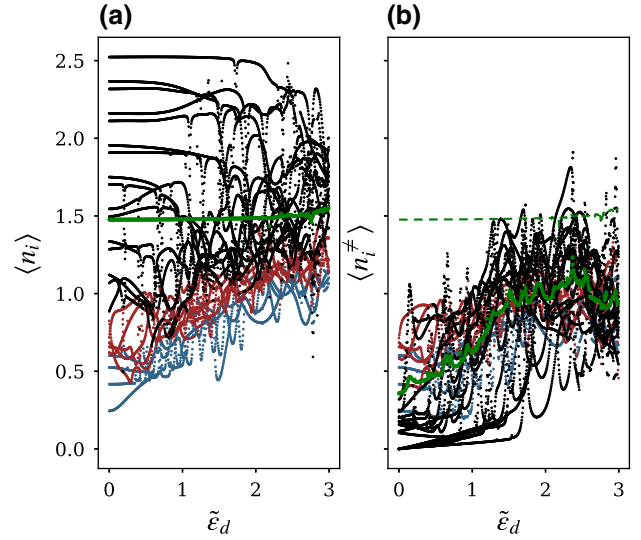
FIG. 16. (a) Mean dipole moment \langle n_i \rangle associated to each Floquet mode i , as a function of the drive amplitude, for the same parameters as in Fig. 1(d), except n_g = 0.12 . The states are sorted through their mean energies. For each Floquet state i , the average in Eq. (E3) is performed over the first 25 transmon states j . For clarity, the low-energy states ( 0 \leq i \leq 3 ) are colored in blue, the states initially close to the separatrix ( 4 \leq i \leq 8 ) appear in red, and the above initially charge-like states are colored in black. The average dipole moment \langle n \rangle is shown in green. Its constant value from \tilde{\epsilon}_d = 0 to 2.5 indicates that higher-energy states do not yet hybridize with the represented states here. For \tilde{\epsilon}_d > 2.5 , we see that \langle n \rangle starts to increase. (b) Same as in (a) but using the definition (E4) for the dipole moment \langle n'_i \rangle , where the average is performed over states with j \neq i . The dipole moment is low for charge-like states until they enter the chaotic layer. The average dipole moment \langle n' \rangle increases with the drive amplitude, due to the increasing number of charge-like states with initially high dipole moment \langle n_i \rangle hybridizing with chaotic states. The average dipole moment \langle n \rangle is plotted for comparison as a green dashed line. At \tilde{\epsilon}_d \approx 2.5 , the states are fully hybridized and \langle n' \rangle is close to \langle n \rangle . For \tilde{\epsilon}_d > 2.5 , hybridization with higher-energy states start to decrease \langle n' \rangle , where the average is performed only on the first 25 states. Besides, the dipole moment of low-energy states \langle n'_i \rangle (in blue) dramatically increase upon entering the chaotic layer.
