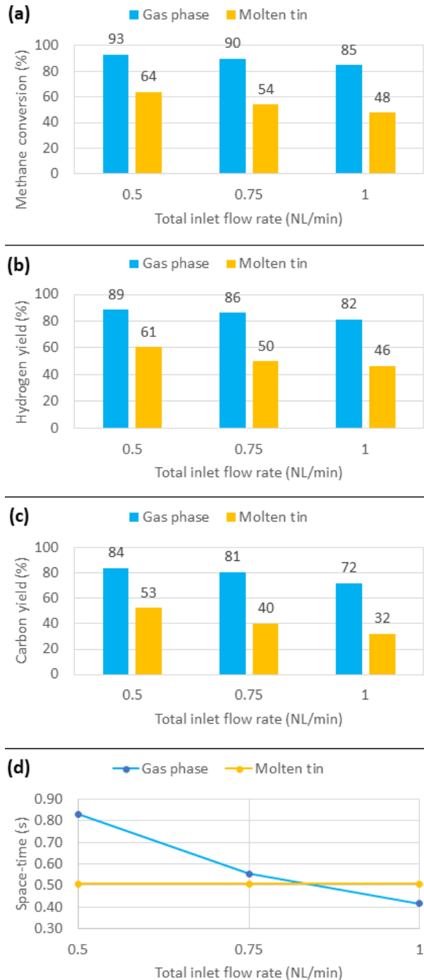
Figure 9: Total inlet flow rate effect on methane pyrolysis in gas phase and in liquid tin with a fixed methane molar fraction of 0.3 and a constant temperature of 1300°C: (a) methane conversion, (b) hydrogen yield, (c) carbon yield, (d) gas space-time in the hot zone of the reactor.
