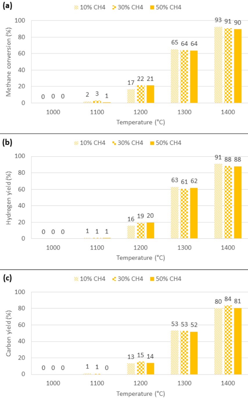
Figure 11: Effect of methane molar fraction on methane conversion and products yields in molten-tin methane pyrolysis: (a) methane conversion, (b) hydrogen yield, (c) carbon yield.
