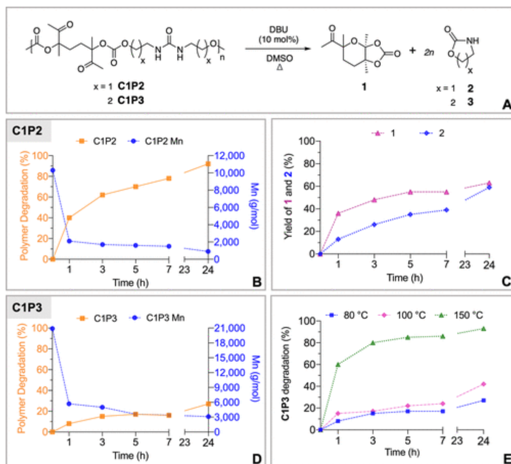
Figure 2. (A) Degradation scheme for C1P2 and C1P3 . (B) Evolution of polymer degradation and M_n of C1P2 with the reaction time at 80 °C. (C) Time evolution of the C1P2 products yields at 80 °C. (D) Time evolution of the C1P3 M_n upon deconstruction at 80 °C. (E) Time evolution of the C1P3 degradation at 80, 100, and 150 °C. The reactions were conducted in the presence of DBU (10 mol % vs polymer repeating unit) using 1,3,5-trimethoxybenzene (TMB) as the internal standard.
