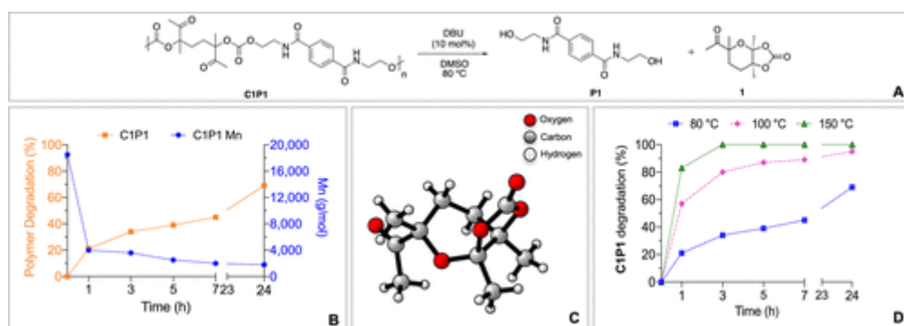
Figure 1. (A) Degradation scheme for C1P1 and main degradation products. (B) Time evolution of the C1P1 M_n upon deconstruction at 80 °C. (C) ORTEP representation of 5-acetyl-3a,5,7a-trimethyltetrahydro-5H-[1,3]dioxolo[4,5- b ]pyran-2-one. (D) Time evolution of the C1P1 degradation at 80, 100, and 150 °C. The reactions were in presence of DBU (10 mol % vs polymer repeating unit) using 1,3,5-trimethoxybenzene (TMB) as an internal standard.
