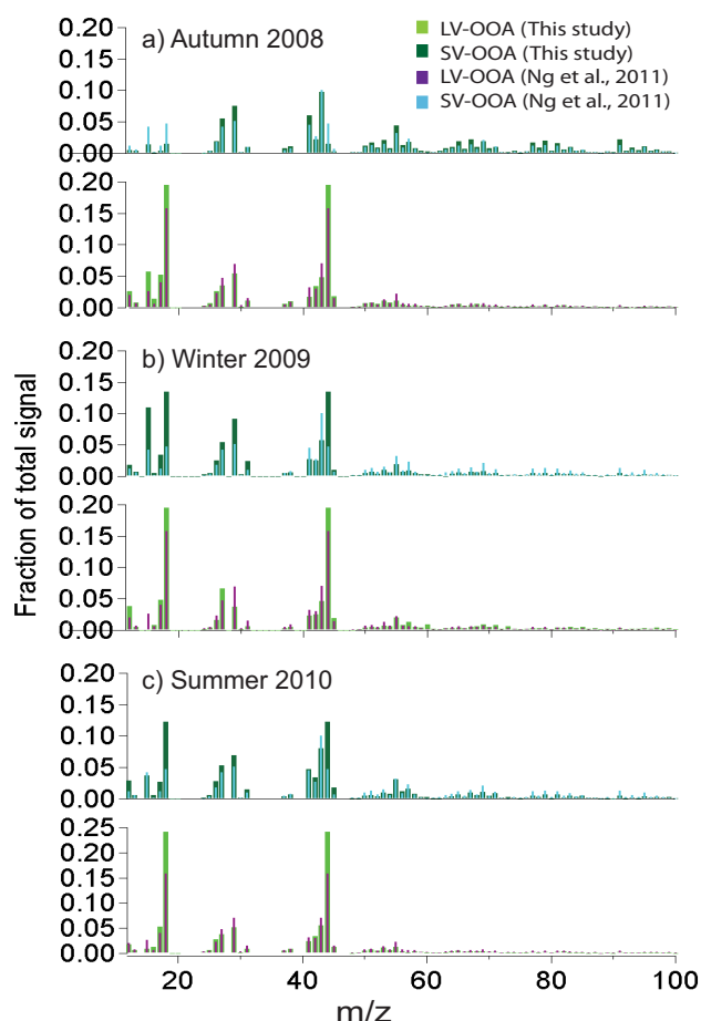
Fig. 3. Average mass spectra of organic species extracted from the total organic mass spectra for the (a) autumn, (b) winter, and (c) summer campaign. Smaller sticks overlayed on each mass spectral pattern represent those of Ng et al. (2011).
