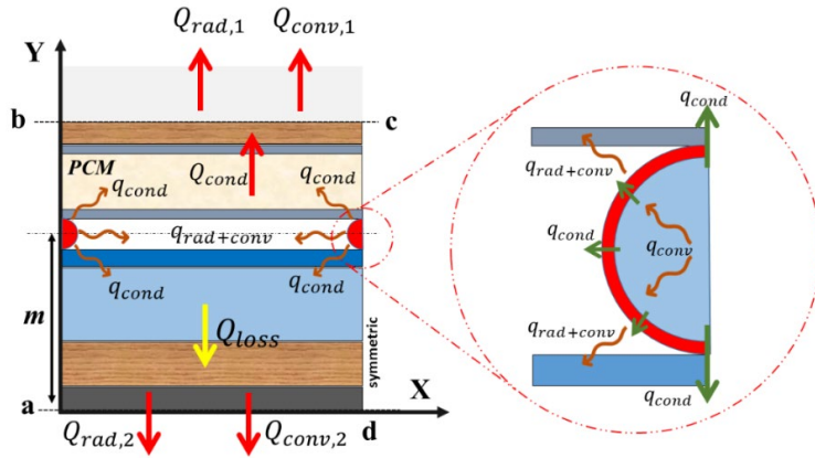
Fig. 4. Detailed cross-section of the floor showing heat transfer within the layers.
