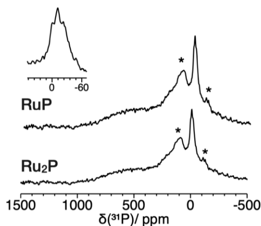
Figure 5. ^{31}\text{P} MAS spectra of RuP (top) and Ru 2 P (bottom). Spectra have been recorded using Hahn echo (HE) sequence. Spinning sidebands are marked with asterisks. The spectral region at low chemical shifts is expanded in the inset of the figure.
