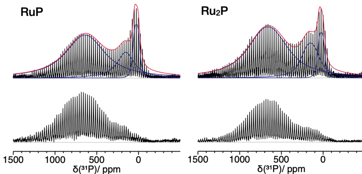
Figure 6. Static ^{31}\text{P} WURST-CPMG spectra of RuP and Ru 2 P. Spectra were recorded with a recycle delay of 5 s (top) and 0.2 s (bottom). For quantitative spectra (top) the spectral fitting is also reported (single peaks in blue and the sum of the three contributions in red).
