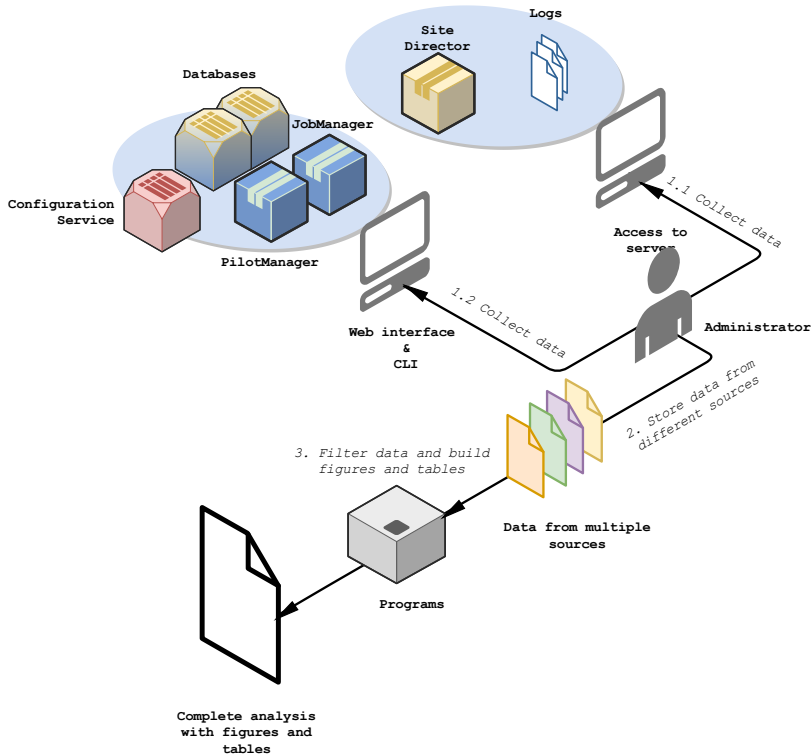
Fig. 2. Workflow: collecting and processing WMS data.
