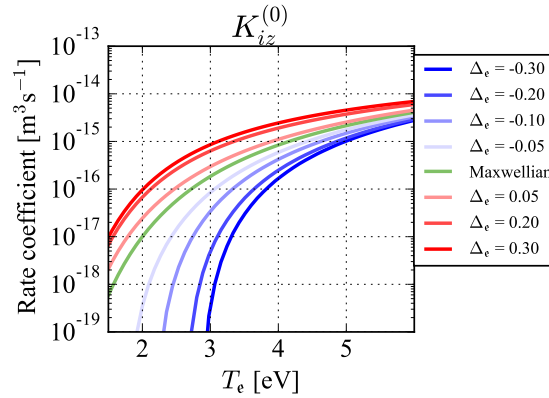
FIG. 3. Influence of the contracted fourth moment on the ionization rate coefficient K_{iz}^{(0)} for argon.
