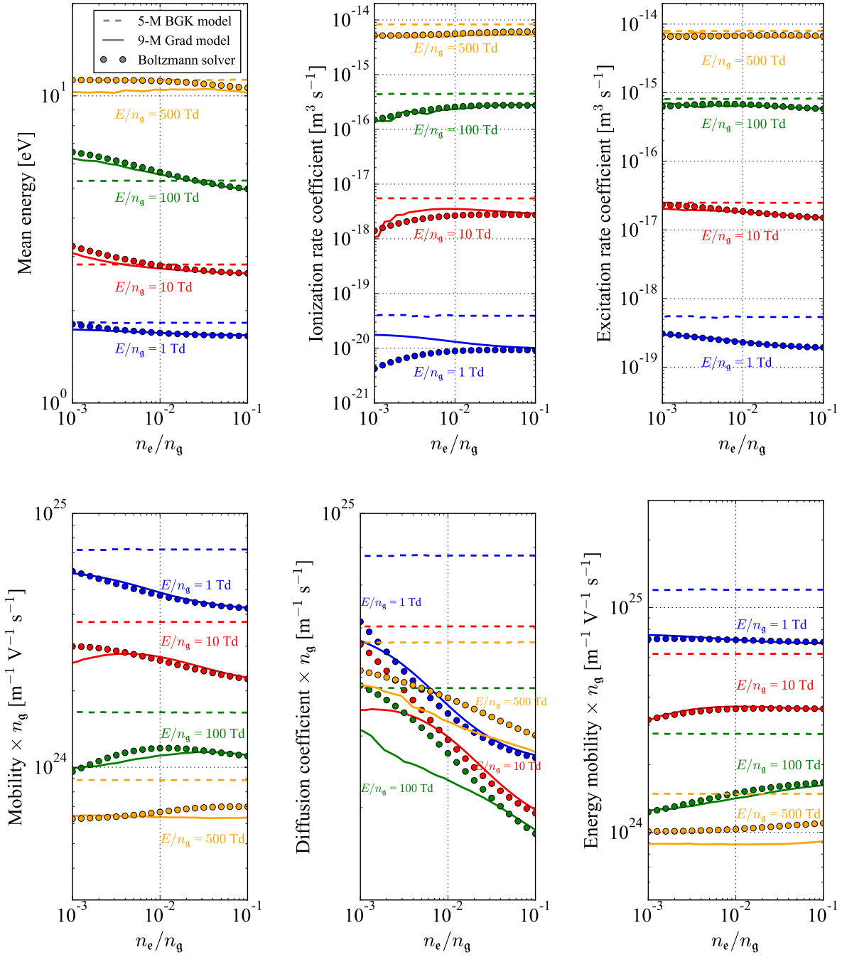
FIG. 11. Comparison of the electron transport coefficients of an argon plasma are computed with a Boltzmann solver and the high-order moment model for different ionization degrees.
