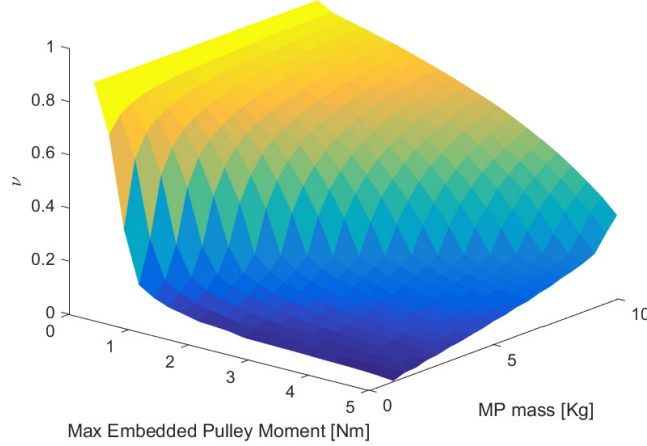
Fig. 7: Ratio v between the areas of the WFW and the surface occupied by the robot in the vertical plane as a function of the MP mass and the maximum moment exerted on the embedded pulley
