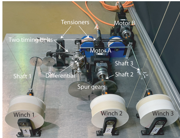
Fig. 10: Photograph of the Transmission system
