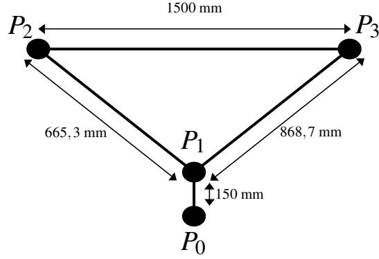
Fig. 14: Path of Trajectory 1 - pure translations and rotations in sequence
