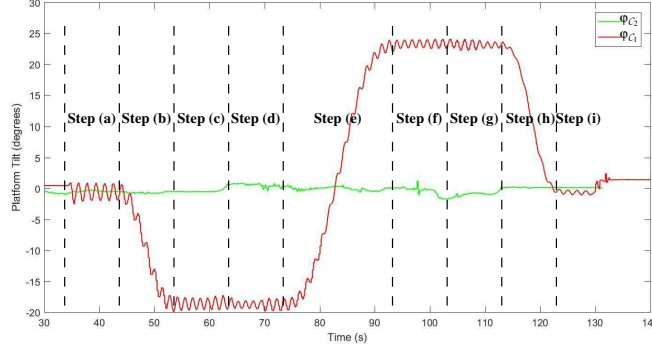
Fig. 16: Tilt angle around axis z_b - Trajectory 1
