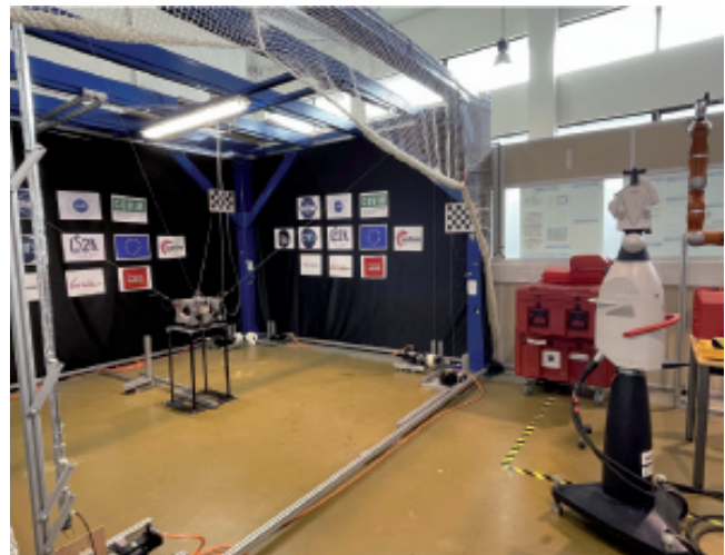
Fig. 1: The complete setup for hardware experiments with the CDPR (left) and the laser tracking system (right).
