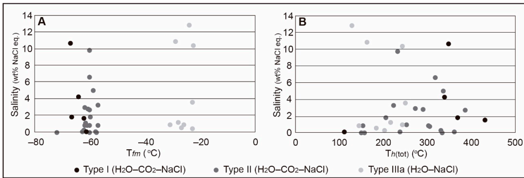
Figure 17. (A) Temperature of first melting ( T_{fm} ) vs. salinity diagram for the fluid inclusions of the Passa Três gold deposit; (B) Total homogenisation temperature ( T_{h-tot} ) vs. salinity plot of the studied fluid inclusions.
