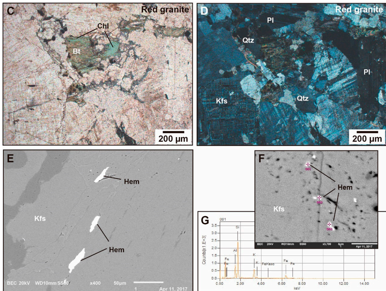
Figure 2. Red granite textures: (A,B) Red granite with medium-grained isotropic texture; biotite crystals altered to chlorite; photographs come from underground mine (A) and from borehole (B); (C,D) Photomicrographs in natural (C) and polarized (D) light of the red granite with biotite altered to chlorite, in a medium-grained isotropic texture (thin section of sample from underground mine); (E) scanning electron microscopy (SEM)/back-scattered electron (BSE) image showing elongated hematite crystals in planes parallel to the K-feldspar cleavage; (F) Hematite crystals in pores of K-feldspar with location of energy-dispersive spectroscopy (EDS) analyses (SEM-BSE image); (G) EDS spectrum indicating the presence of Fe in the inclusions analysed. Abbreviations: Bt—biotite; Chl—chlorite; Hem: hematite; Kfs—K-feldspar; Pl—plagioclase; Qtz—quartz.
