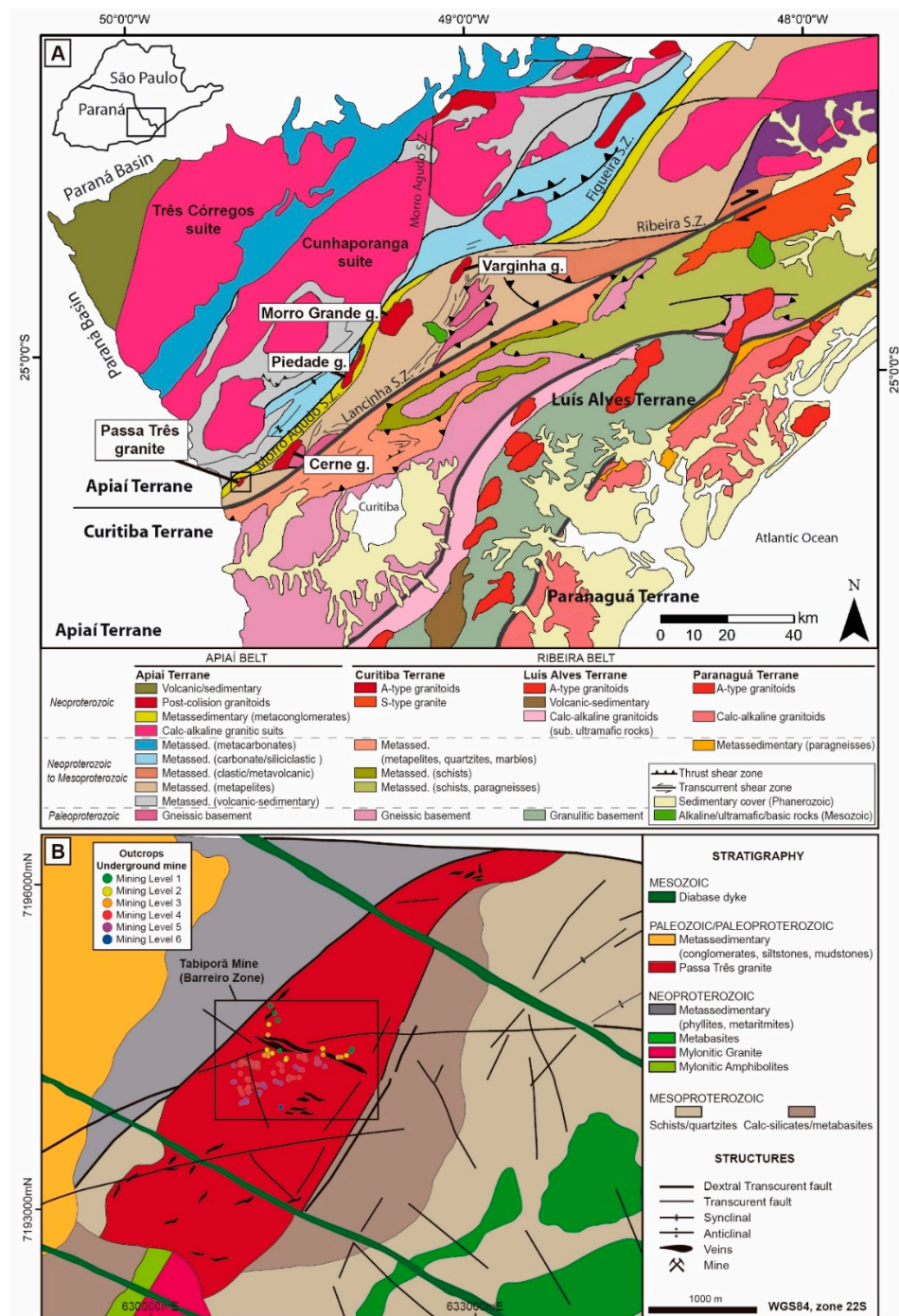
Figure 1. (A) Geological map of the Eastern Paraná State with localisation of the Passa Três granite; the Apiaí, Curitiba, Luís Alves, and Paranaguá terranes are also indicated with limits marked by a grey thick line (adapted from [43]); (B) Local geological map of Passa Três granite and surrounding rocks (adapted from [15]) with indication of the sample’s location by mine level.
