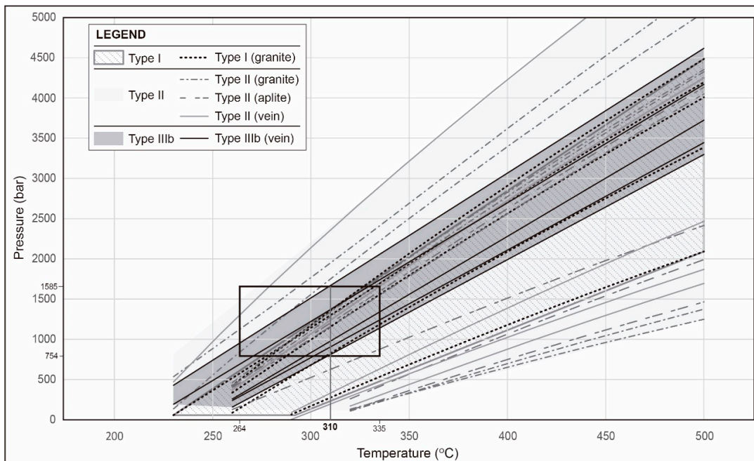
Figure 19. Pressure–temperature (P-T) diagram with isochores of the different fluid inclusion types in the Passa Três gold deposit. The black rectangle represents entrapment conditions of mainly type IIIb fluid inclusions, those associated with the mineralisation stage, and constraints from chlorite geothermometry (temperatures of formation from 264 to 335 °C; average temperature of 310 °C).
