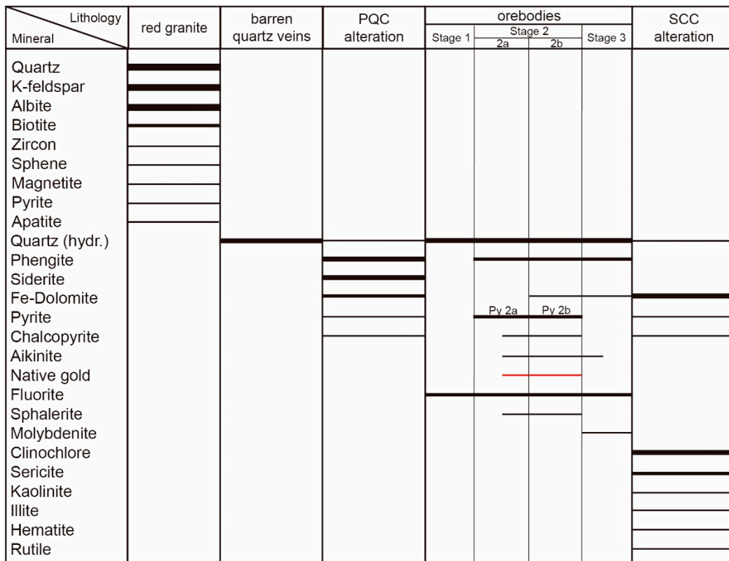
Figure 7. Paragenetic sequence of the red granite, barren quartz veins, mineralized veins, and hydrothermal alteration at the Passa Très gold deposit. The width of the solid lines denotes the relative abundance of minerals. The late argillic alteration in the deposit is not indicated. Criteria for differentiation between phengite and sericite is based on grain size.
