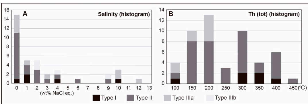
Figure 18. Frequency diagram of (A) salinities and (B) T_{h-tot} of the fluid inclusion types studied in the Passa Três deposit.
