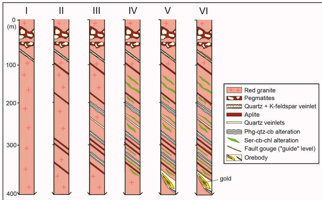
Figure 20. Schematic diagram of drill holes showing the evolutionary model of formation and distribution of the main alteration zones and mineralised veins. Different stages represent chronological order of events. Abbreviations: Cb—carbonate; Chl—chlorite; Phg—phengite; Qtz—quartz; Ser—sericite.
