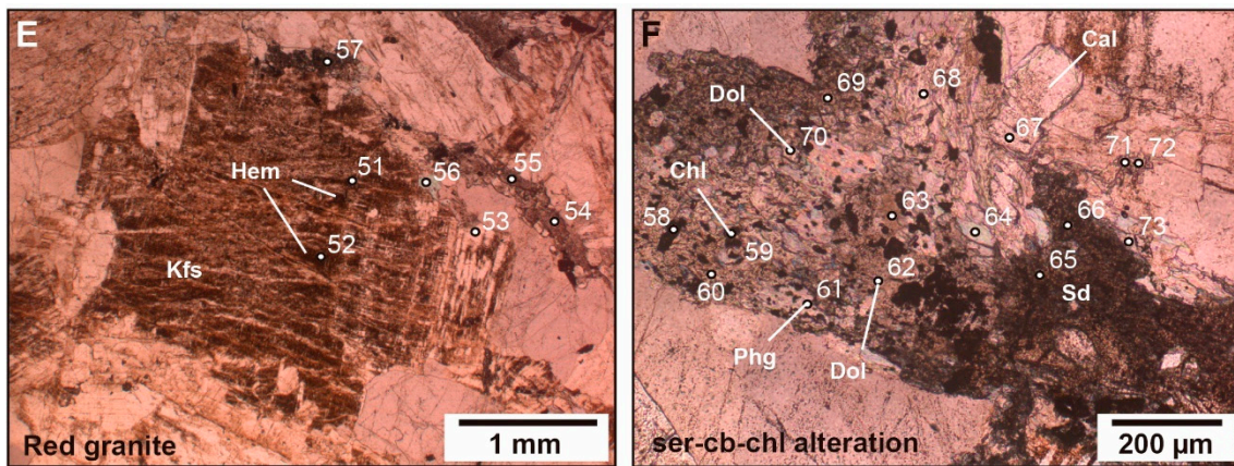
Figure 12. Thin section photomicrographs of SCC alteration minerals of the Passa Trés granite analysed by EPMA: (A) Chlorite replacing magmatic biotite; (B) Mafic aggregate in red granite formed by biotite and altered amphibole; analytical points indicate the presence of clinocllore, siderite (Fe(Mg) carbonate), Fe-dolomite (Ca-Mg-Fe carbonate), and calcite as alteration minerals; (C) Fe-dolomite (Ca-Mg-Fe carbonate) and siderite (Fe(Mg) carbonate) as alteration in the red granite; (D) Relic sphene crystal altered to siderite (Fe(Mg) carbonate), phengite, Fe-dolomite (Ca-Mg-Fe carbonate), and rutile, SCC alteration; (E) K-feldspar with Fe-oxide exsolution as indicated by the presence of FeO in the EPMA analysis; (F) Biotite replaced by clinocllore, calcite, Fe-dolomite, siderite, sericite (phengite), with indication of the points of analyses. Images (A–F): optical microscope—natural light. Abbreviations: Cal—calcite; Cb—carbonate; Chl—chlorite; Dol—Fe-dolomite; Hem—hematite; Kfs—K-feldspar; Phg—phengite; Qtz—quartz; Sd—siderite; Ser—sericite.
