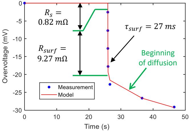
Figure 4: Example of parameters extraction from the beginning of a GITT result for the studied cell (discharging pulse at C/20 , 5^\circ\text{C} , between SoC 62.5% and 87.5%).
