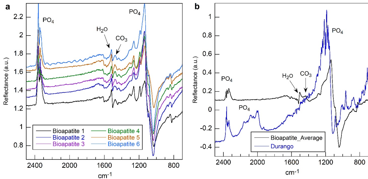
Figure S9. Infrared spectra measured in reflection mode of six bioapatites for 16GC-470 (a) and Durango apatite powder together with the average spectrum of the six bioapatites (b). A CO 3 peak is observed on the bioapatite spectra and not on the Durango apatite spectrum. The reflection peaks of PO 4 at 1000-1100 cm -1 and H 2 O near 1500 cm -1 resemble a first derivative of a Gaussian peak, because the intensity of reflection is determined by the refractive index which has a minimum and a maximum on either side of the absorption bands (Yamamoto and Ishida, H. (1994) Optical theory applied to infrared spectroscopy. Vibrational spectroscopy , 8, 1-36).
