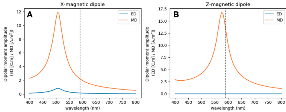
Fig. 8. Spectral decomposition of the internal field response of the core structure to an MD excitation with a dipolar moment amplitude of 1 \text{ A.m}^2 (A) oriented along the x -axis (in-plane) and (B) along the z -axis (out of plane). The vertical dashed black lines stand for the optimized wavelength of emission \lambda_m = 590 \text{ nm} .
