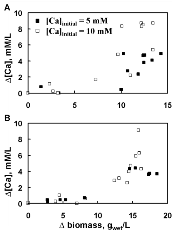
Fig. 7. Relationship between the amount of precipitated Ca (mM/L) and increase of the biomass ( \text{g}_{\text{wet}}/\text{L} ) in biotic experiments with Rhodovulum steppense A-20s (A) and Rhodovulum sp. S-17-65 (B) in nutrient solution. Initial experimental conditions: [\text{Ca}] = 5 and 10 mM; [\text{DIC}] = 5 - 20 mM. Data from Bundeleva et al. (2012).
