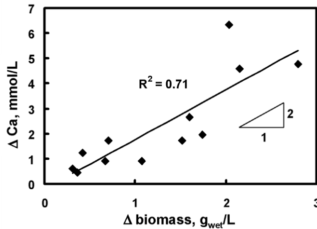
Fig. 6. Relationship between the amount of precipitated Ca (mM/L) and increase of the biomass ( \text{g}_{\text{wet}}/\text{L} ) in biotic experiments with Gloeocapsa sp. in nutrient solution. Experimental conditions: \Omega initial = 15-150; pH = 8.6-9.6.
