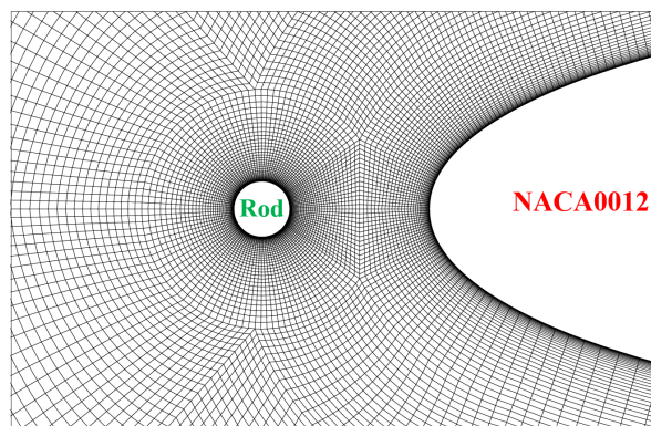
FIGURE 7 – Generated mesh for NACA0012 aerofoil controlled by micro-cylinder rod.
