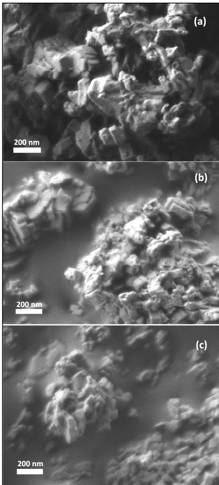
Fig. 3 SEM micrographs in the magnitude 50000x of Fe-Cu-Z (a), K-Fe-Cu-Z (b) and Na-Fe-Cu-Z (c).
