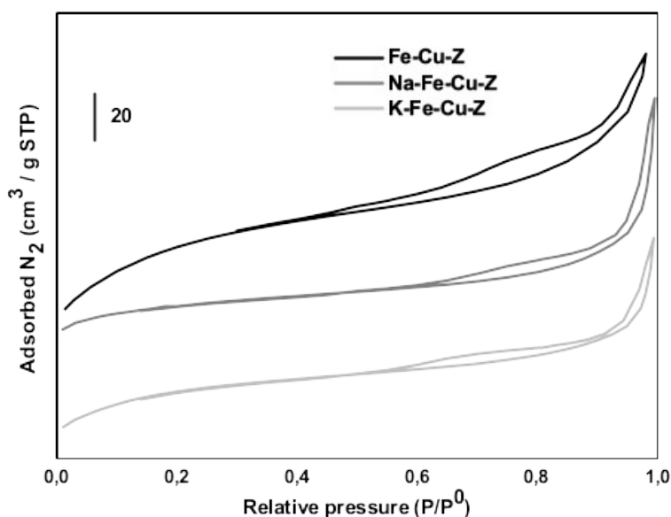
Fig. 2 N 2 Adsorption-desorption isotherms of prepared catalysts.
