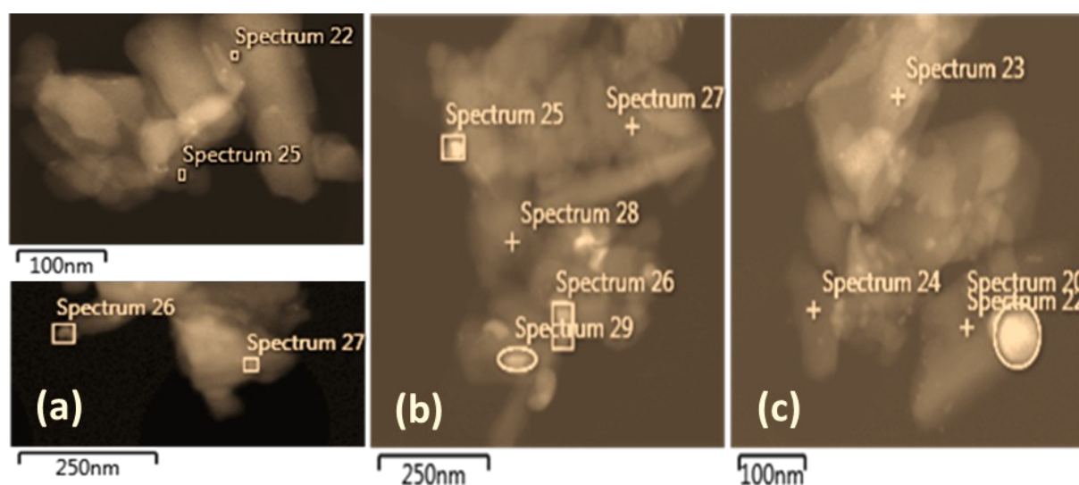
Fig. 4 STEM micrographs of Fe-Cu-Z (a), K-Fe-Cu-Z (b) and Na-Fe-Cu-Z (c).
