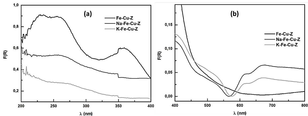
Fig. 5 DRS UV-vis spectra of studied catalysts
