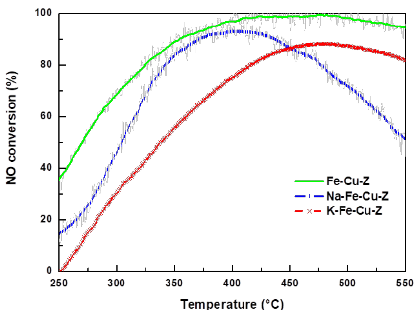
Fig.7 NO conversion over the prepared catalysts.
