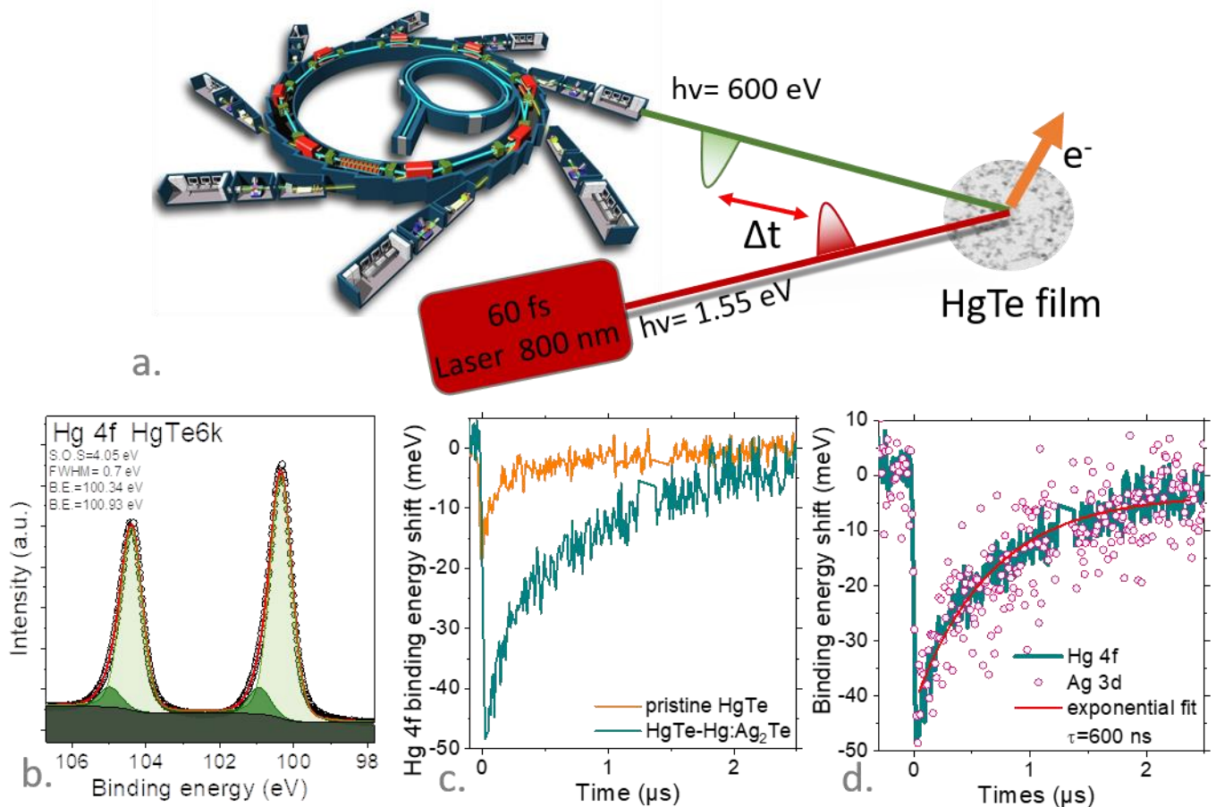
Figure 2 a. Schematic of the pump probe photoemission. fs laser at 800 nm is used to excite the NC film and soft X-rays from synchrotron are used as a probe ( h\nu=600 \text{ eV} ). b. Photoemission spectrum from the Hg 4f state. c. Binding energy of the Hg 4f 7/2 state after a pulse of light ( t=0 ) at 800 nm from a pristine HgTe NC film and from the same film covered with Hg exchanged Ag 2 Te thin layer. d. Binding energy shift of the Hg 4f 7/2 state and Ag 3d 5/2 state after a pulse of light ( t=0 ) at 800 nm from a HgTe NC film covered with Hg exchanged Ag 2 Te thin layer. All measurements are made at room temperature, while samples are deposited on a gold substrate.
