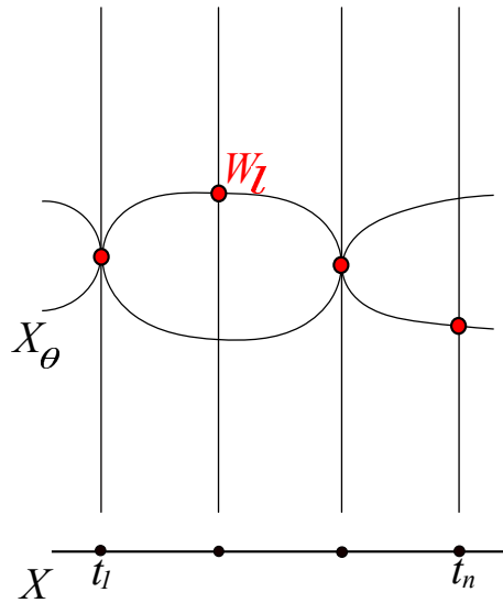
FIGURE 1. Divisor W_l defined by parabolic directions.
