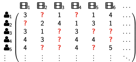
Figure 1: Rating matrix / table containing users' ratings for the movies
